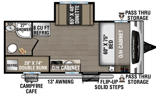
SL169VUD UVW – 3,720 lbs. | Exterior Length – 21' 11" | Sleeps – 6
